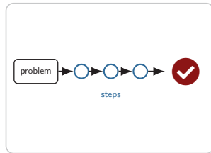
Reasoning models
